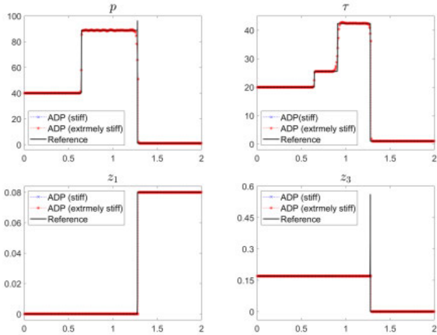
FIG. 4.12. Example 9b: Pressure ( p ), temperature ( \tau ), mass fraction of H_2 ( z_1 ) and mass fraction of OH ( z_3 ) computed by the stiff and extremely stiff ADP methods for 1/\varepsilon_1 = 1/\varepsilon_2 = 10^7 .
