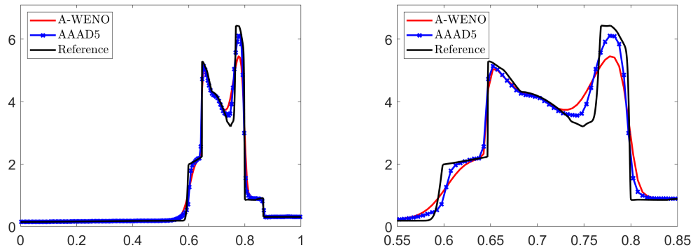
FIG. 4.11. Example 6: Density \rho computed by the A-WENO and AAAD5 schemes with \Delta x = 1/200 (left) and zoom at x \in [0.55, 0.85] (right).
