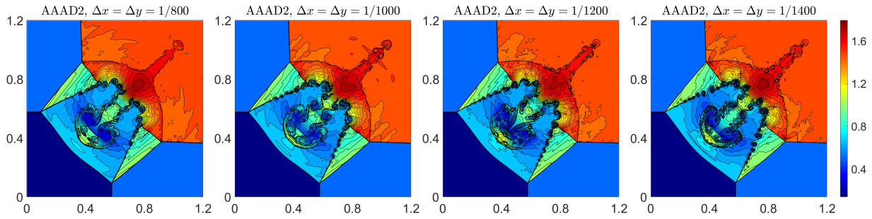
FIG. 4.15. Example 9: Density \rho computed by the AAAD2 scheme on uniform meshes with \Delta x = \Delta y = 3/2000, 3/2500, 1/1000 , and 3/3500 with \mathcal{C} = 0.04 .
