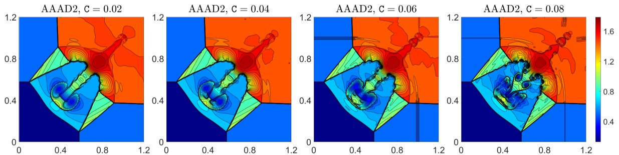
FIG. 4.14. Example 9: Density \rho computed by the AAAD2 scheme with \Delta x = \Delta y = 3/1000 for \mathcal{C} = 0.02, 0.04, 0.06 , and 0.08 .
