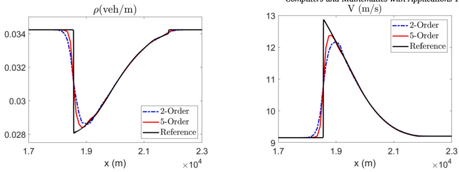
Fig. 13. §4.3.2, Test 1: Density (left) and speed (right) computed by the 2-Order and 5-Order Schemes.
