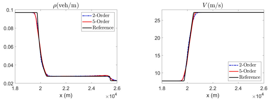
Fig. 10. §4.3.1, Test 7: Same as in Fig. 4.
