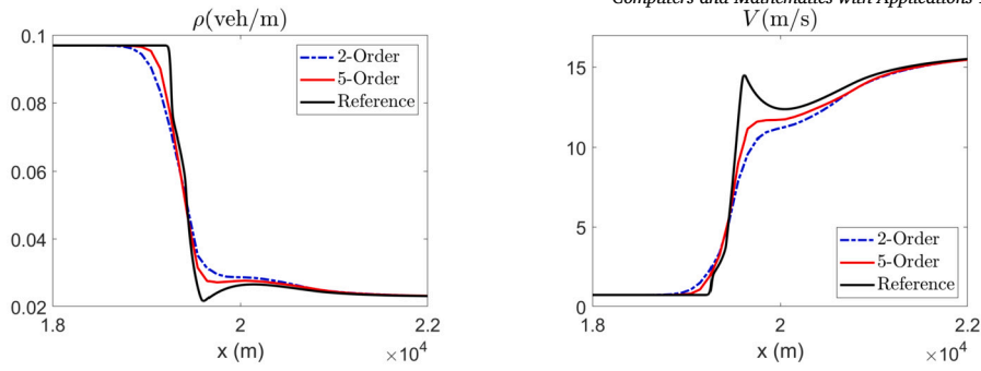
Fig. 17. §4.3.2, Test 5: Same as in Fig. 13.
