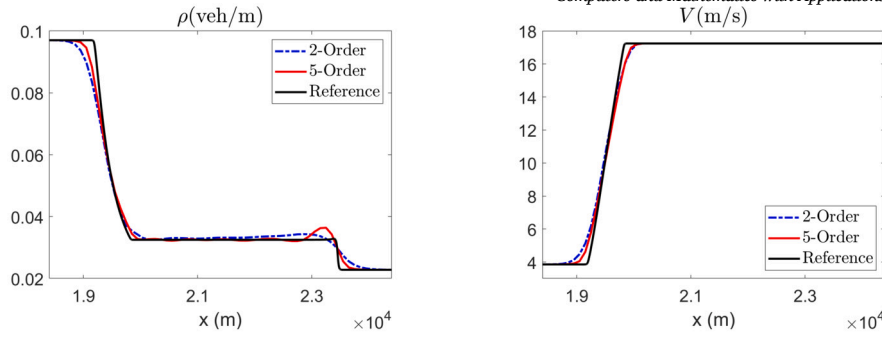
Fig. 11. §4.3.1, Test 8: Same as in Fig. 4.
