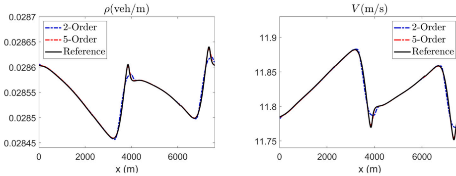
Fig. 22. §4.4, Test 9: Density (left) and speed (right) computed by the 2-Order and 5-Order Schemes.
