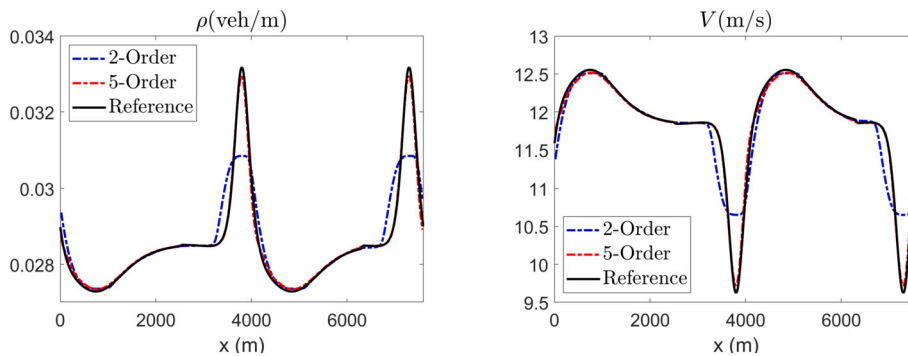
Fig. 23. §4.4, Test 10: Same as in Fig. 22.
