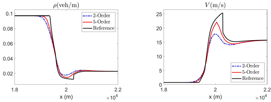
Fig. 18. §4.3.2, Test 6: Same as in Fig. 13.
