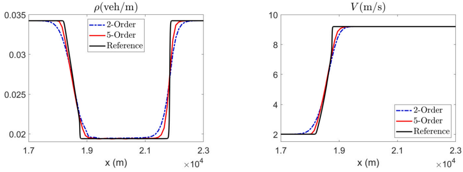
Fig. 4. §4.3.1, Test 1: Density (left) and speed (right) computed by the 2-Order and 5-Order Schemes.
