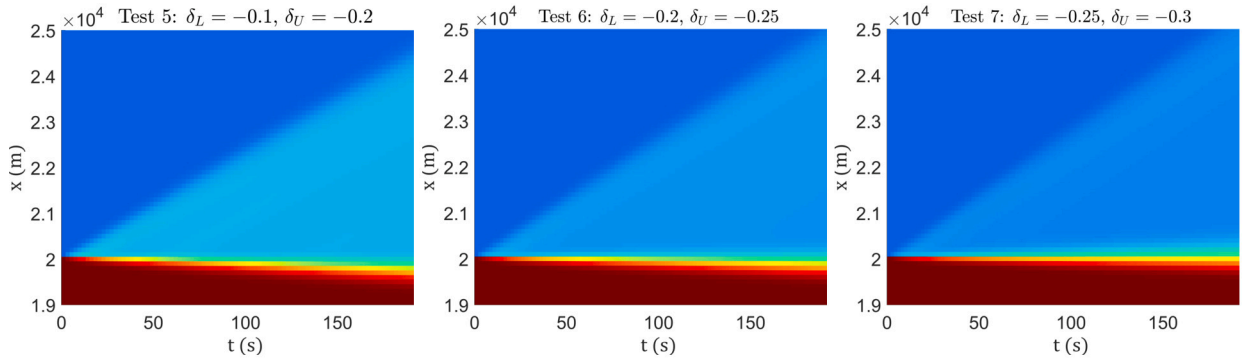
Fig. 12. Spatio-temporal evolution of traffic density for Tests 5–7 with the same initial data but different risk perception parameters. With a decrease in \delta_L and \delta_U (from left to right), drivers' perception of risk and alertness increase, and they respond to the traffic conditions ahead quicker. Consequently, traffic waves propagate quicker.
