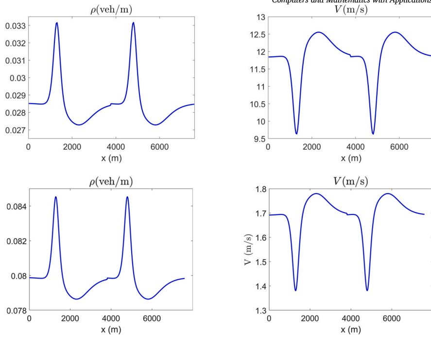
Fig. 21. §4.4: Initial conditions for Tests 9 and 10 (top row) and Test 11 (bottom row).
