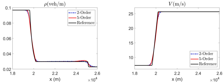
Fig. 9. §4.3.1, Test 6: Same as in Fig. 4.
