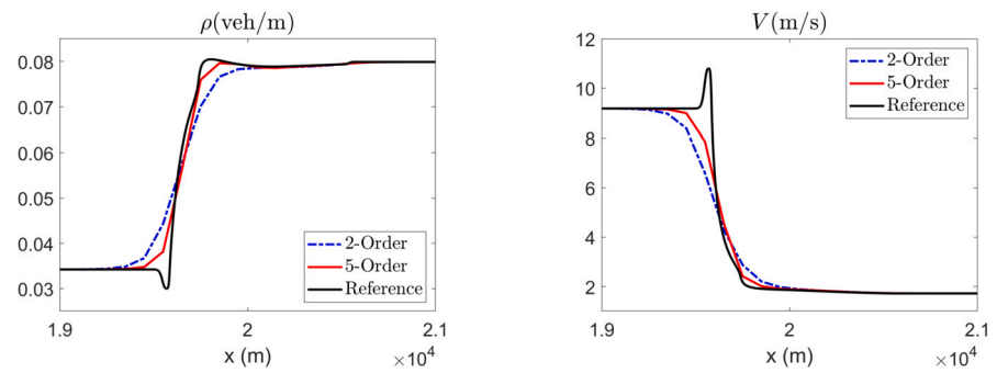
Fig. 16. §4.3.2, Test 4: Same as in Fig. 13.
