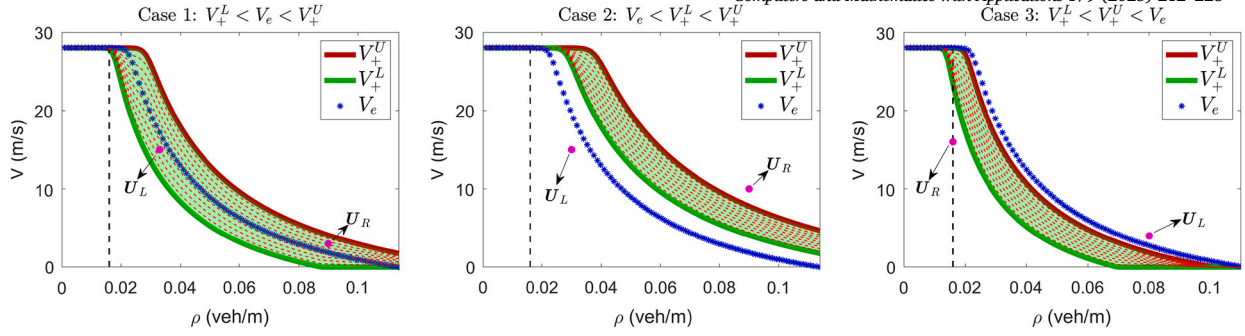
Fig. 2. Three different possibilities for the status of the U_L and U_R in the speed-density plane.
