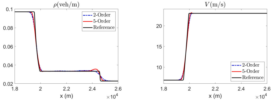
Fig. 8. §4.3.1, Test 5: Same as in Fig. 4.
