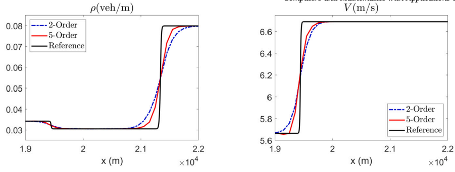
Fig. 7. §4.3.1, Test 4: Same as in Fig. 4.
