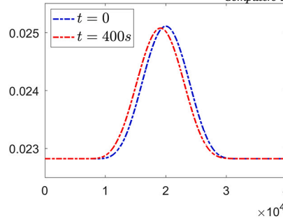
Fig. 1. Accuracy test: Density ( \rho ) profiles at t = 0 and 400 s computed by the 2-Order scheme.
