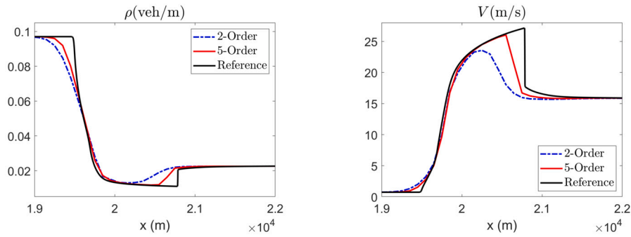
Fig. 19. §4.3.2, Test 7: Same as in Fig. 13.
