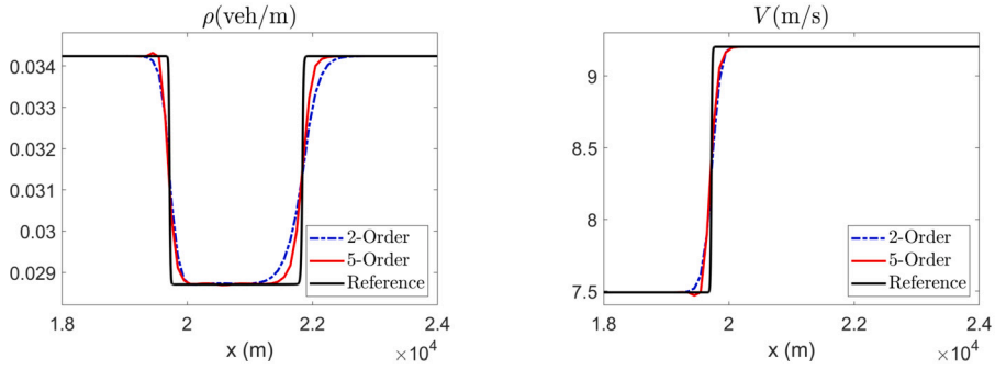
Fig. 5. §4.3.1, Test 2: Same as in Fig. 4.
