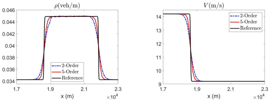
Fig. 6. §4.3.1, Test 3: Same as in Fig. 4.
