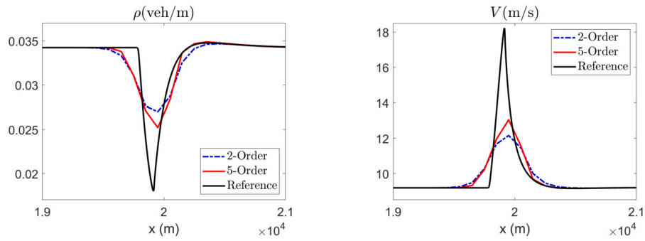
Fig. 14. §4.3.2, Test 2: Same as in Fig. 13.
