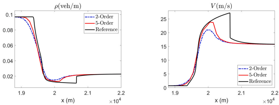
Fig. 20. §4.3.2, Test 8: Same as in Fig. 13.
